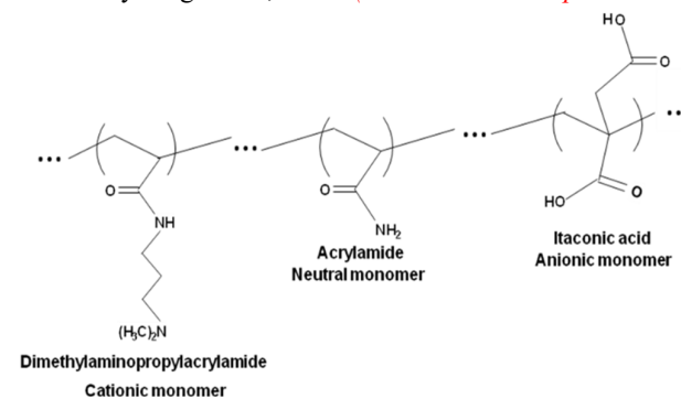
Figure 1 - Polyampholyte molecular composition prepared by random, free-radical polymerization. (Bold, size 10)
